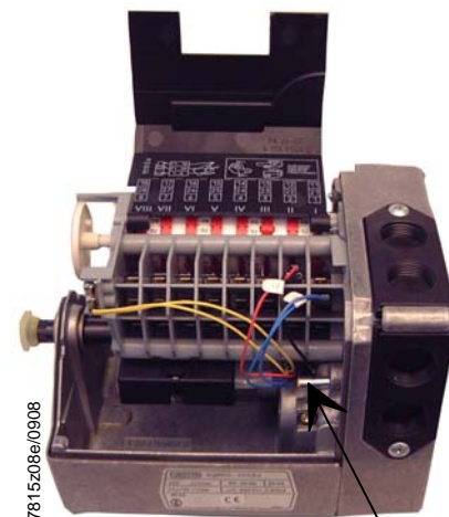
Pressure pin "K1"
