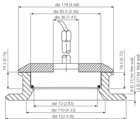
Fig. 29 - Sanitary seal with flush diaphragm
