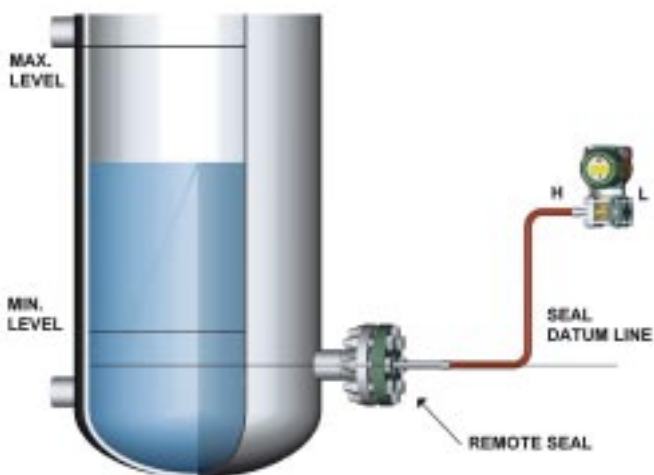
Fig. 4 - Level measurement of a liquid in an open tank
