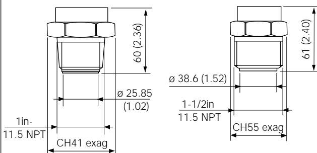
Fig. 41 - Threaded connection
