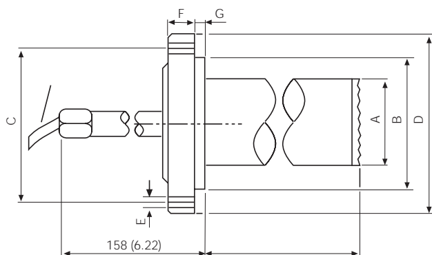
Fig. 14 - Extended diaphragm remote seal
