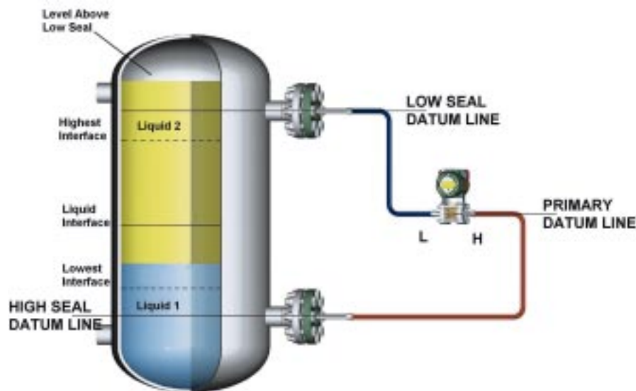
Fig. 9 - Interface level measurement
