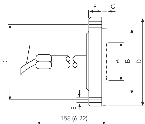
Fig. 15 - Flanged flush diaphragm remote seal
