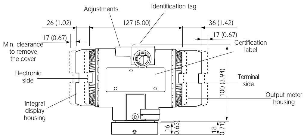
Fig. 37 - 264HP/NP housing. Common part for all the following spuds and connections
