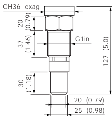
Fig. 42 - Ball valve connection
