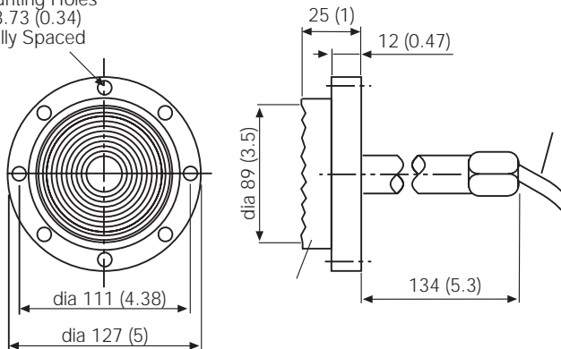
Fig. 13 - Chemical Tee remote seal
