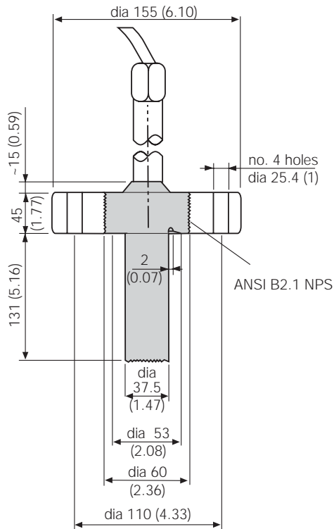
Fig. 17 - Remote seal for Urea Service
