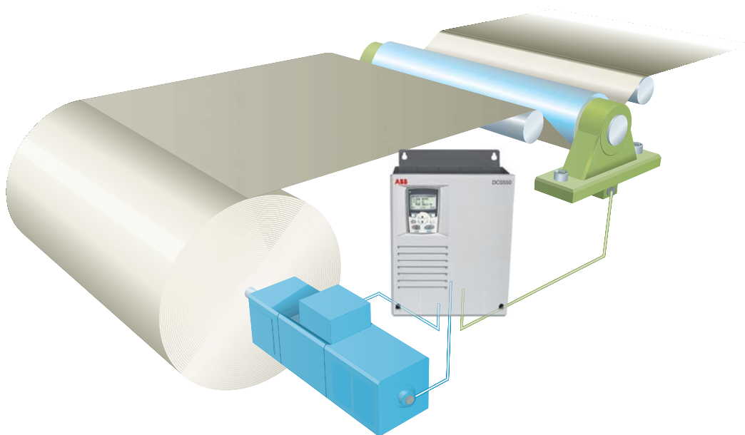
Example: direct tension control (closed loop)
